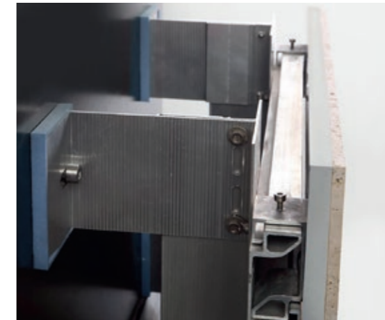
System detail for ventilated facades
