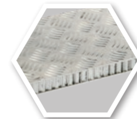
COMPOCEL AL FLOOR COMPOCEL AL FR FLOOR* Upper face chosen among different antiskid/ anti-slip coatings. Lower skin: raw aluminium.
